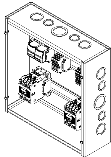
PERSPECTIVE VIEW
