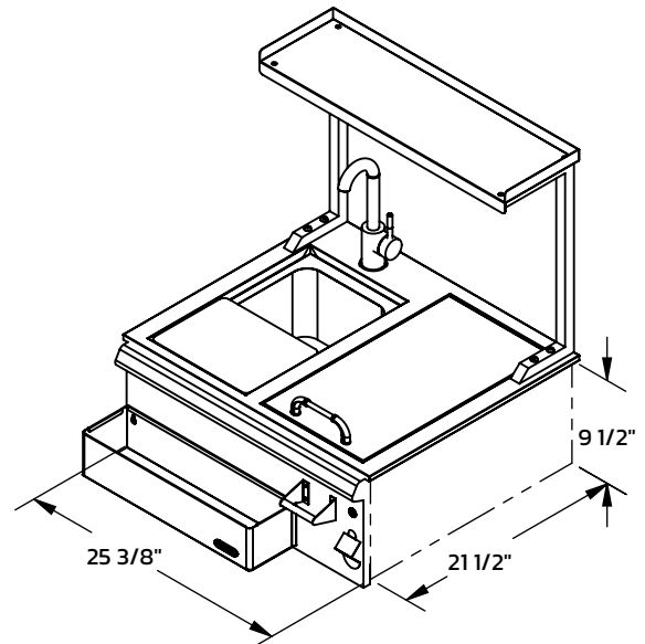
ISOMETRIC TOP VIEW WITH INSTALLATION CUT OUT DIMENSIONS
