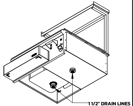
ISOMETRIC BOTTOM VIEW DRAIN LINE DETAILS
